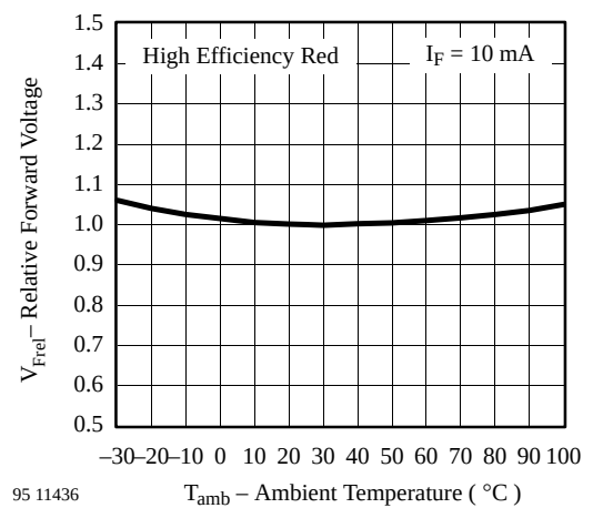
Figure 3. Relative Forward Voltage vs. Ambient Temperature
