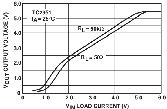
Figure 2. Dropout Characteristics
