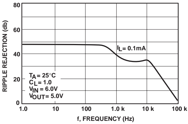
Figure 11. Ripple Rejection
