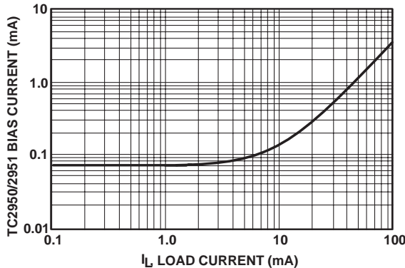
Figure 1. Quiescent Current
