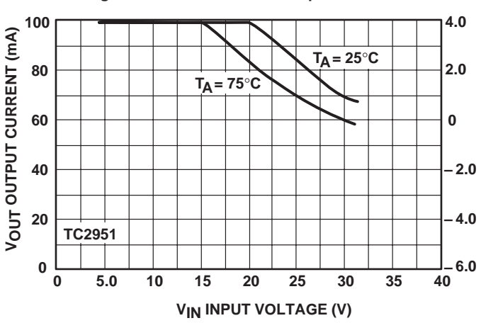
Figure 14. Maximum Rated Output Current
