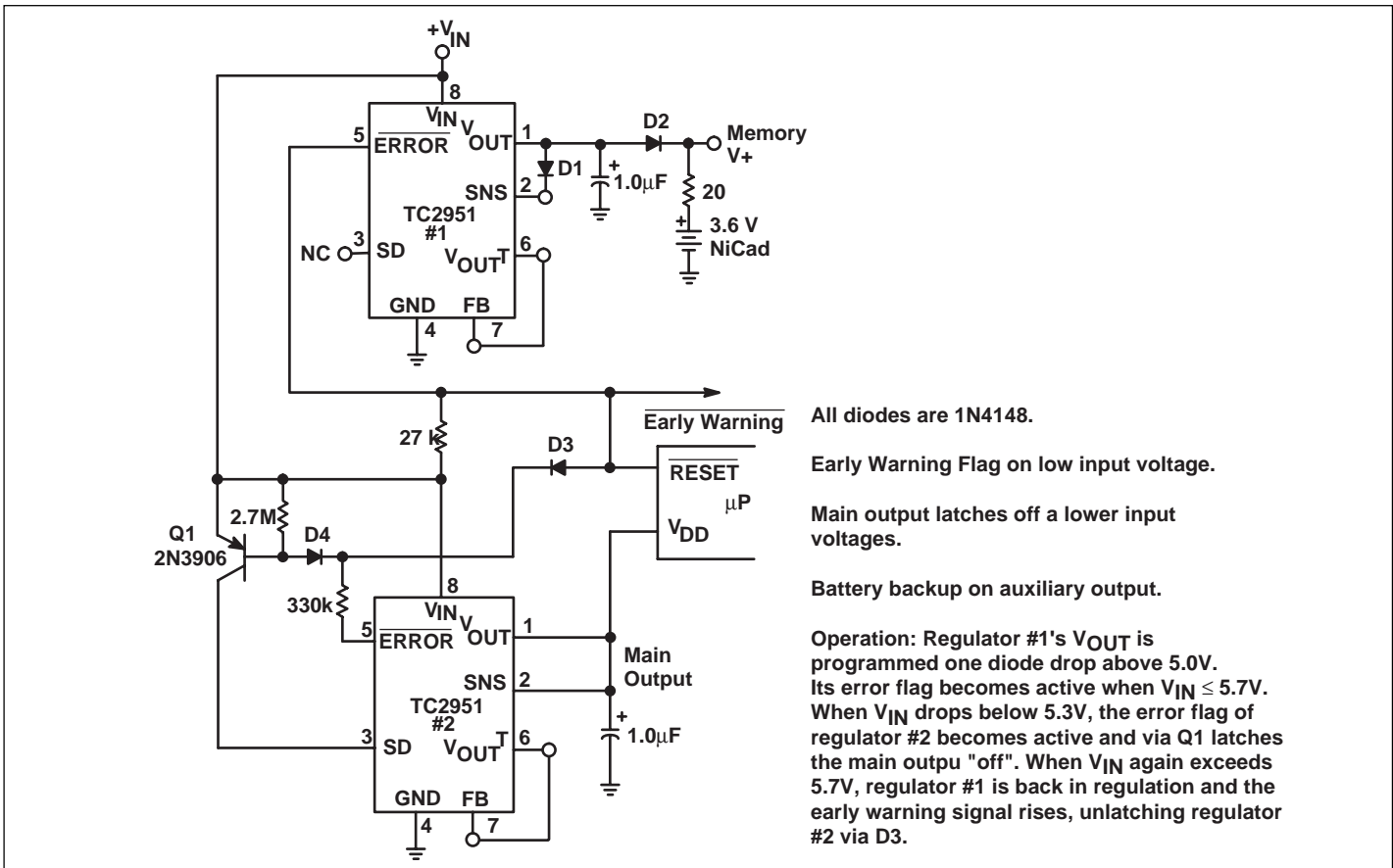
Figure 22. 5.0V Regulator with Early Warning and Auxiliary Output
