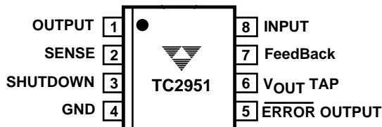
8-Pin SOIC
