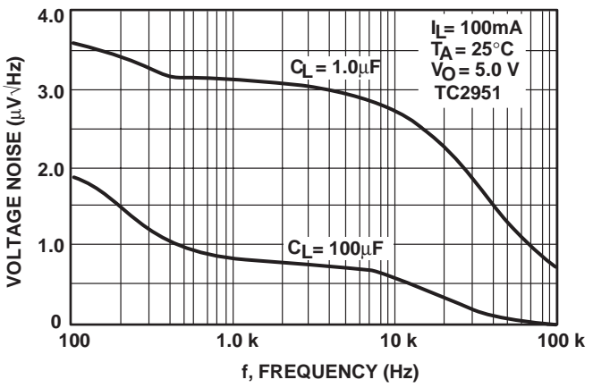
Figure 12. Output Noise
