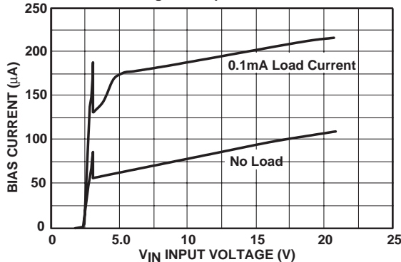
Figure 3. Input Current
