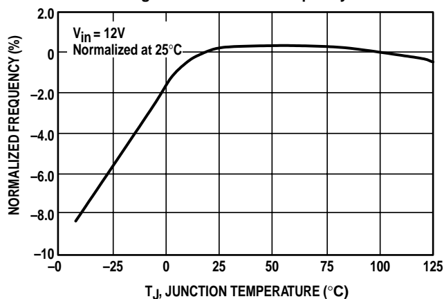
Figure 28. Oscillator Frequency
