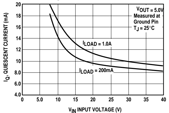
Figure 25. Quiescent Current
