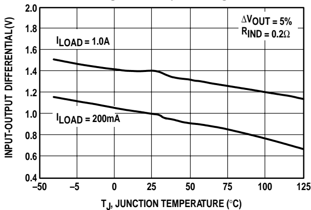
Figure 24. Dropout Voltage
