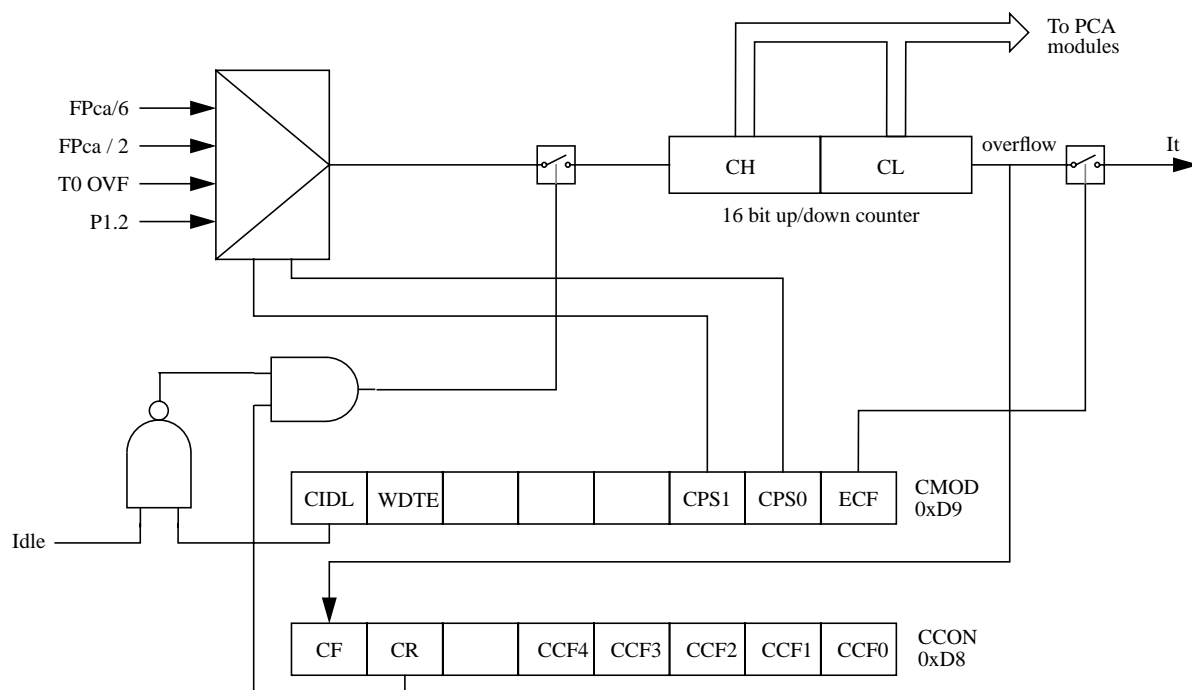
Figure 115. PCA Timer/Counter
