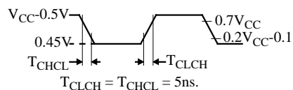
Figure 147. Clock Signal Waveform for I_{CC} Tests in Active and Idle Modes
