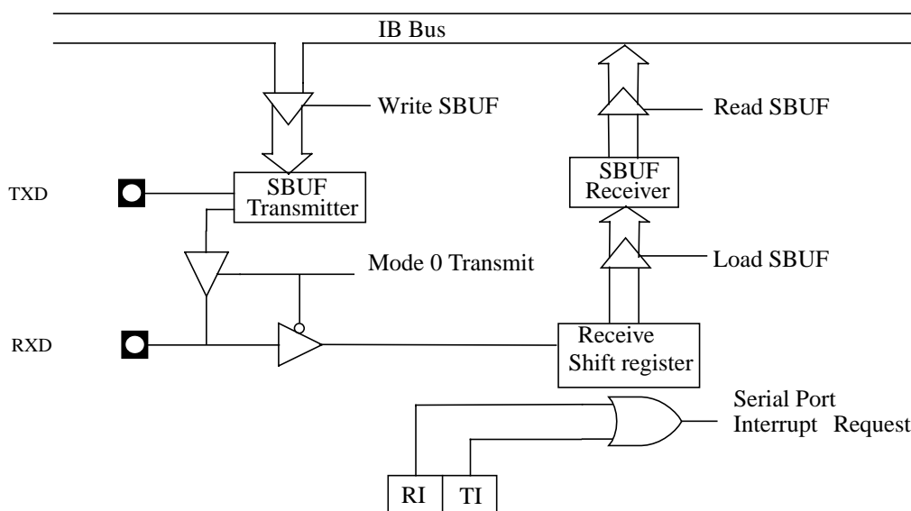
Figure 33. Serial I/O Port Block Diagram
