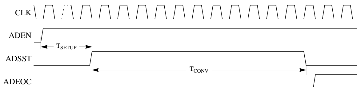
Figure 129. Timing Diagram
