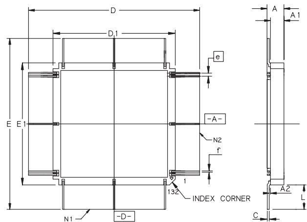
Figure 2: 132 pins MQFPF
