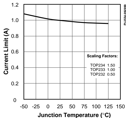
EXTERNAL CURRENT LIMIT vs. TEMPERATURE with R_M = 12K \Omega
