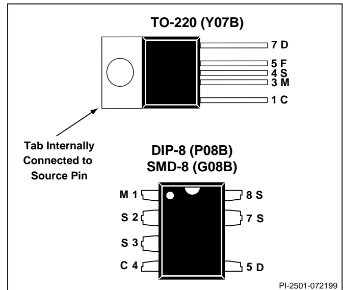
Figure 3. Pin Configuration.
