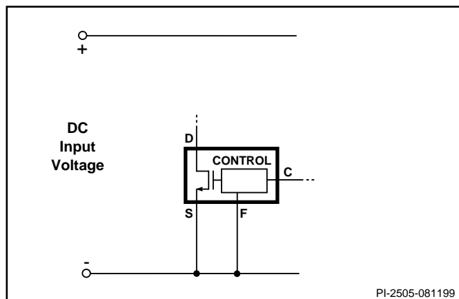
Figure 10. Full Frequency Operation (130 kHz).
