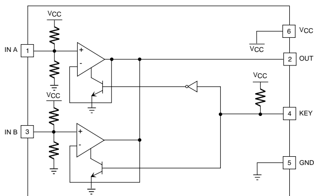
BLOCK DIAGRAM
