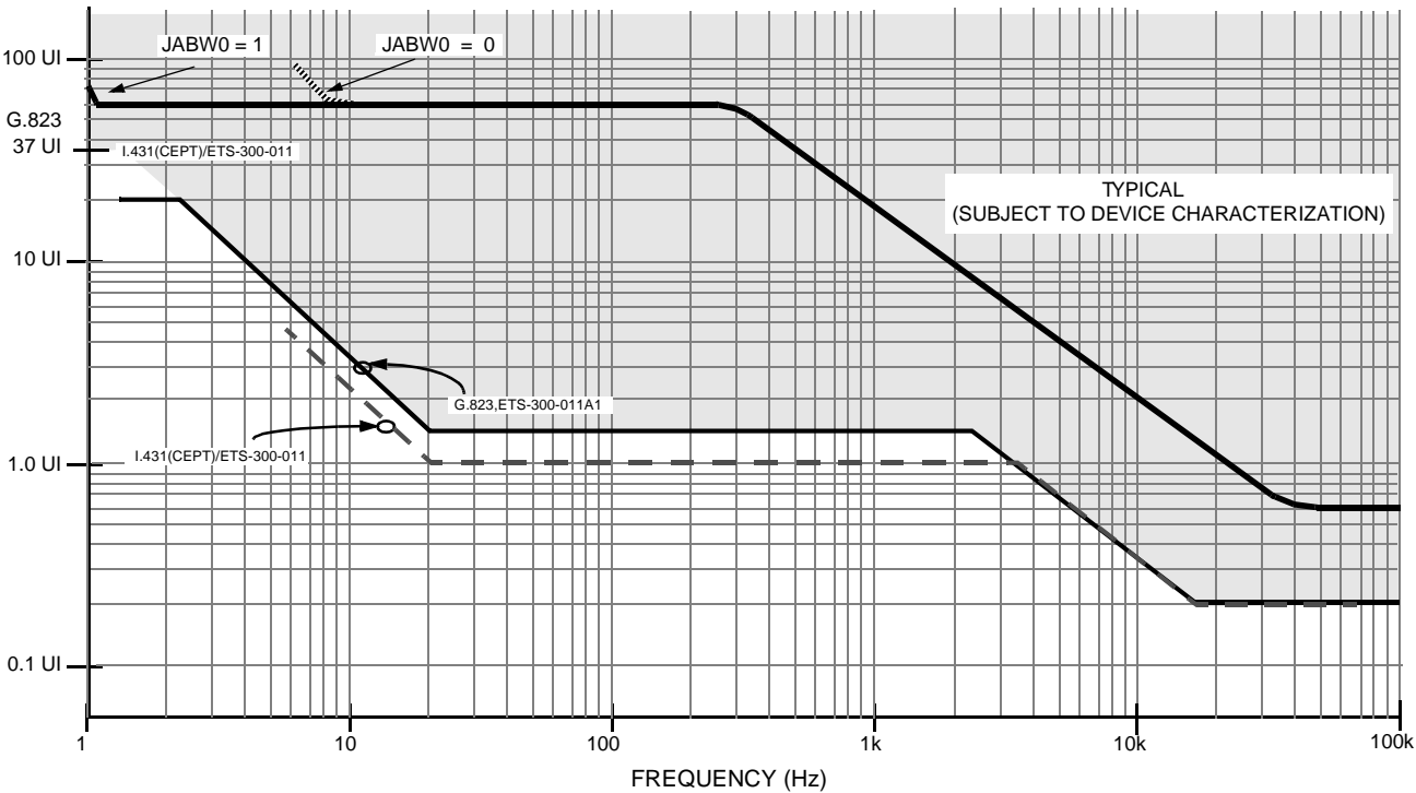
Figure 14. CEPT/E1 Receiver Jitter Accommodation with Jitter Attenuator
