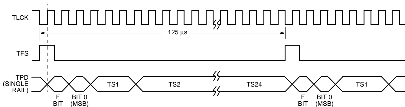
Figure 31. Timing Specification for TFS, TLCK, and TPD in DS1 Mode
