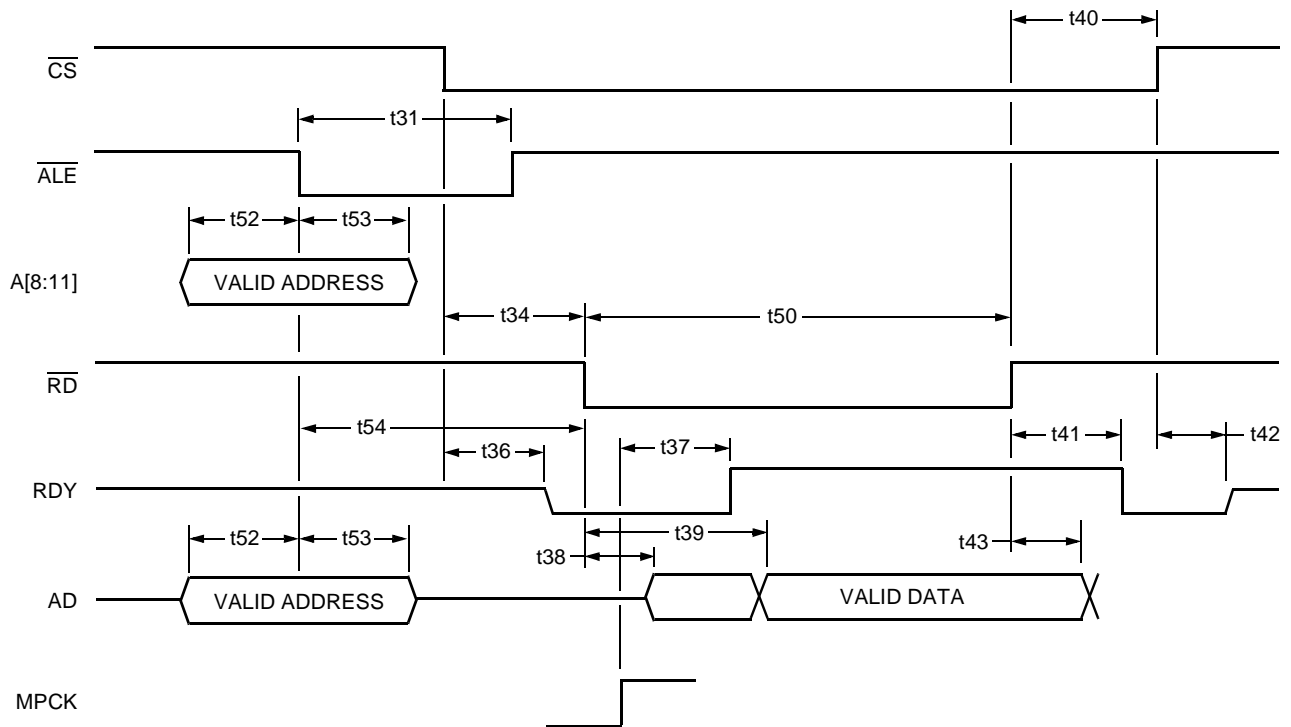
Figure 65. Mode 4—Read Cycle Timing (MPPMODE = 1, MPMUX = 1)
