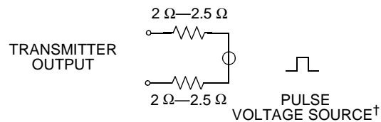
B. Transmitter Output Approximate Equivalent Circuit
