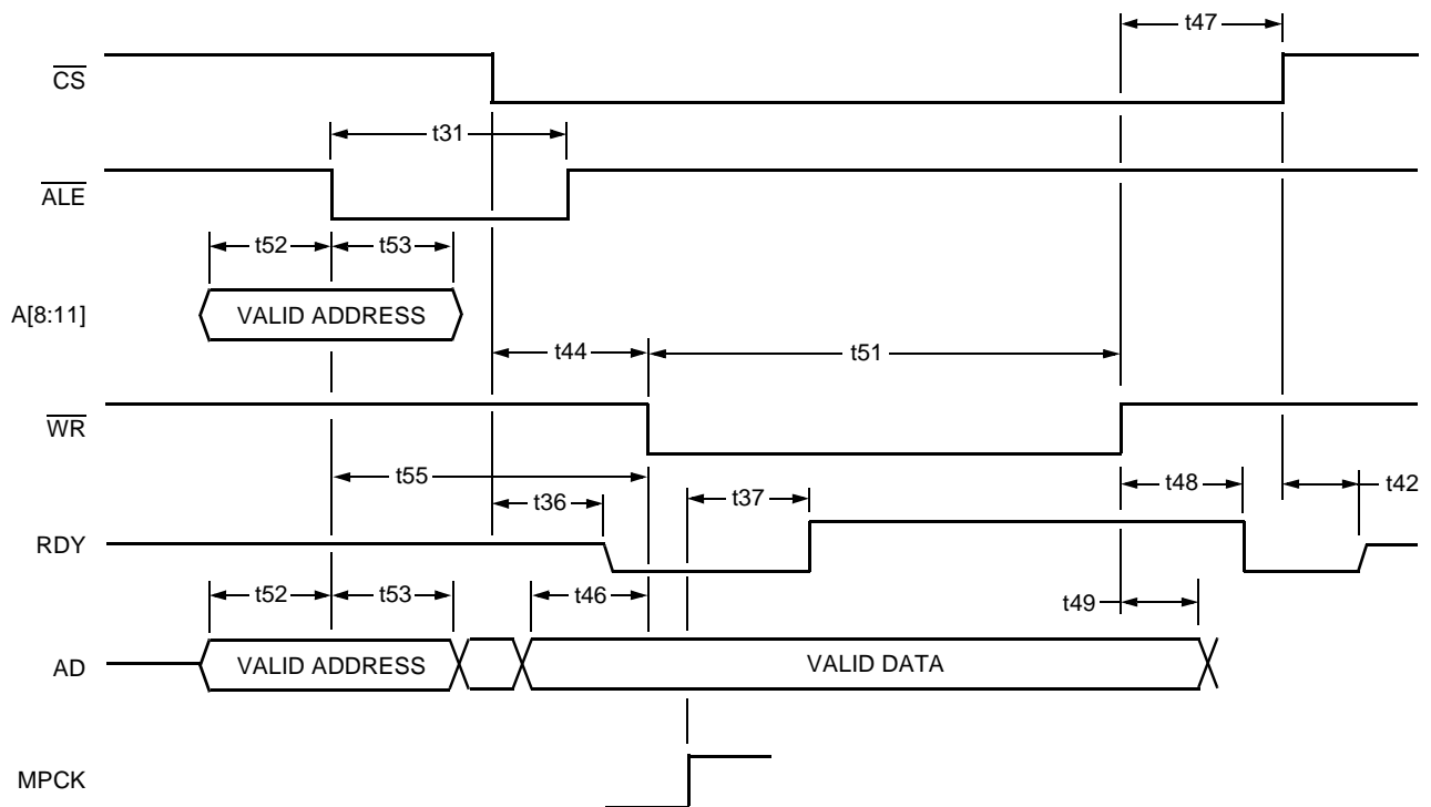
Figure 66. Mode 4—Write Cycle Timing (MPPMODE = 1, MPMUX = 1)
