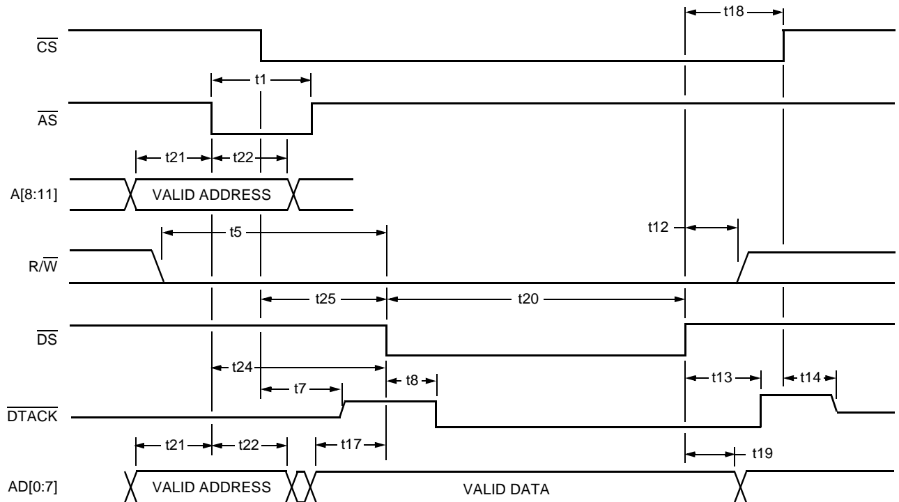
Figure 62. Mode 2—Write Cycle Timing (MPPMODE = 0, MPMUX = 1)
