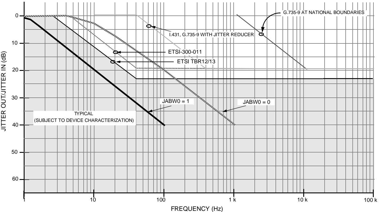
Figure 15. CEPT/E1 Jitter Transfer of the Jitter Attenuator
