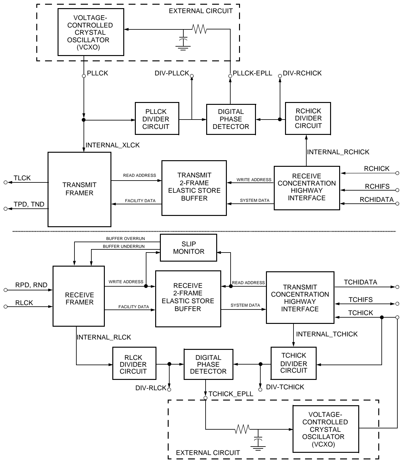
Figure 49. T7630 Phase Detector Circuitry
