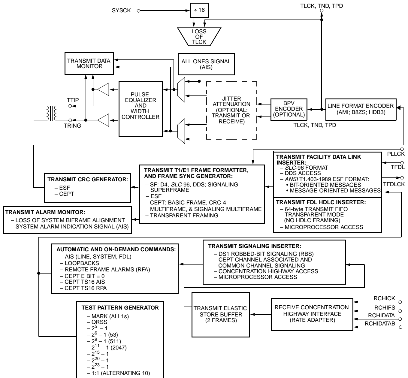
Figure 3. T7630 Block Diagram: Transmit Section (One of Two Channels)
