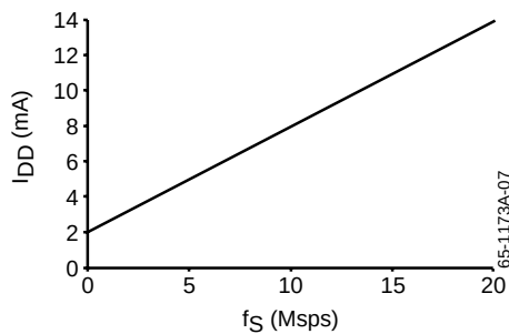
Figure 8. Typical I_{DD} vs f_S
