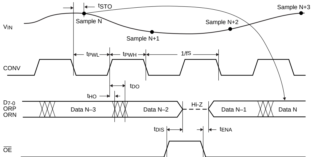
Figure 2. Conversion Timing
