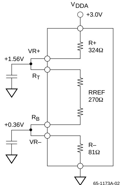
Figure 1. Reference Resistors
