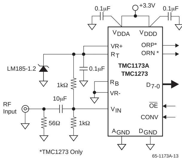
Figure 14. Stabilized Reference Circuit
