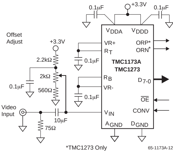
Figure 13. Low Cost Circuit
