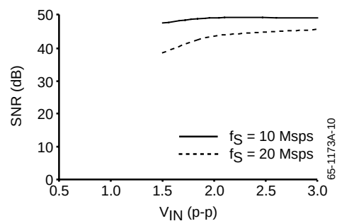
Figure 11. Typical SNR vs Full Scale Input Range
