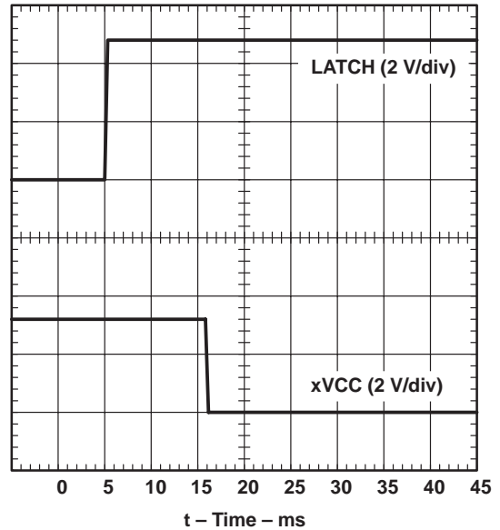
Figure 4. xVCC Propagation Delay and Fall Time With 1-μF Load, 3.3-V Switch, V_{I(5V)} = 5V
