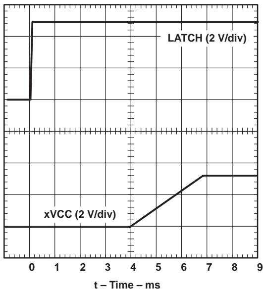
Figure 5. xVCC Propagation Delay and Rise Time With 150-μF Load, 3.3-V Switch, V_{I(5V)} = 5V
