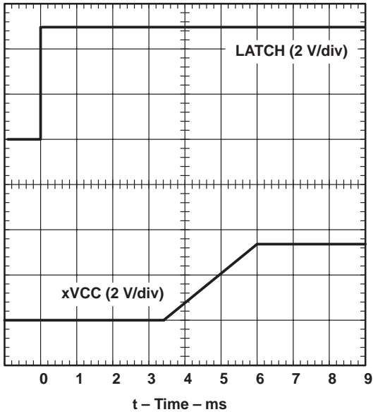
Figure 3. xVCC Propagation Delay and Rise Time With 1-μF Load, 3.3-V Switch, V_{I(5V)} = 5V
