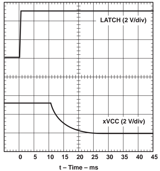
Figure 6. xVCC Propagation Delay and Fall Time With 150-μF Load, 3.3-V Switch, V_{I(5V)} = 5V
