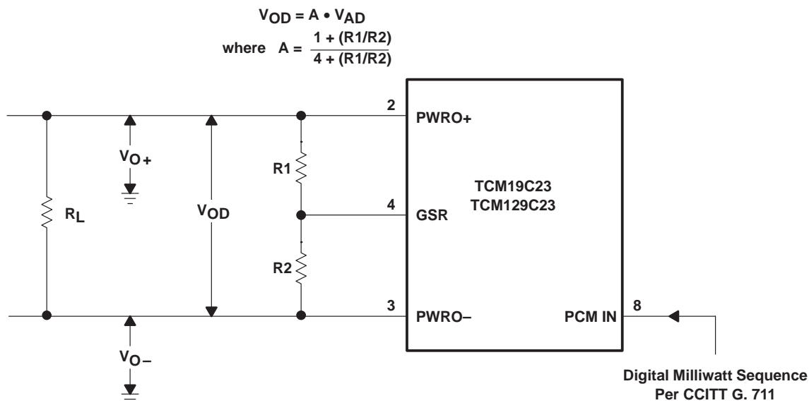
Figure 8. Gain-Setting Configuration
