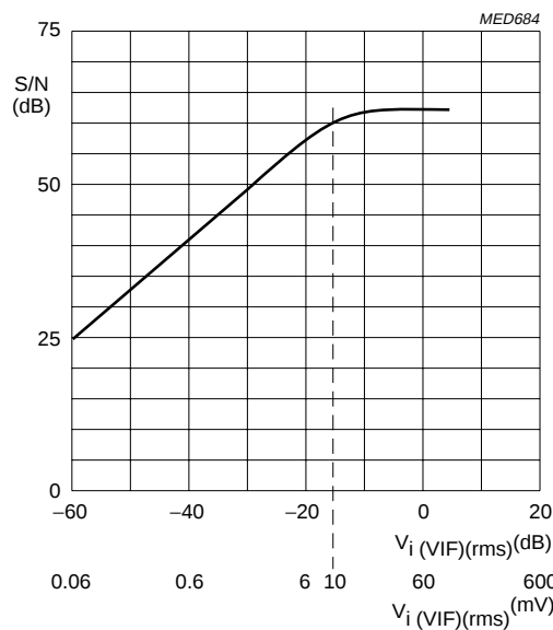
Fig.6 Typical signal-to-noise ratio as a function of IF input voltage.
