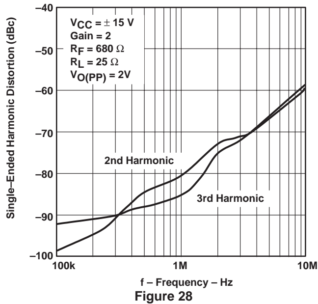
SINGLE-ENDED HARMONIC DISTORTION VS FREQUENCY
