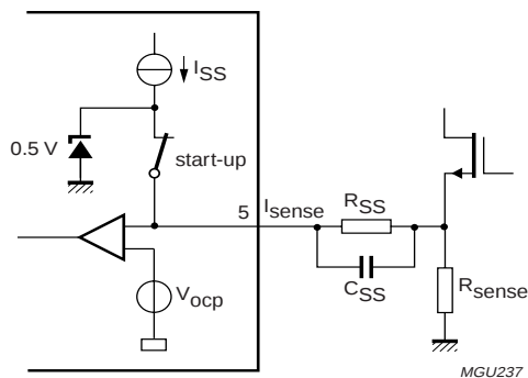
Fig.10 Soft start.
