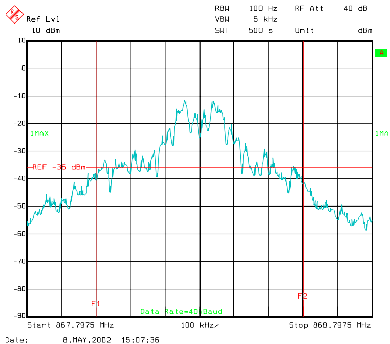
Figure 4-13 FSK Transmit Spectrum 40kBaud, Manch, PRBS9, 9dBm, 3V
