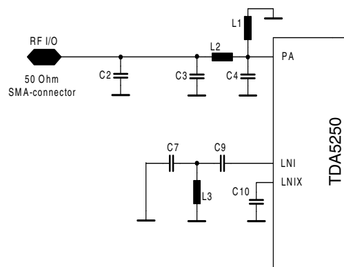
Figure 4-5 TX_Mode_simplified
