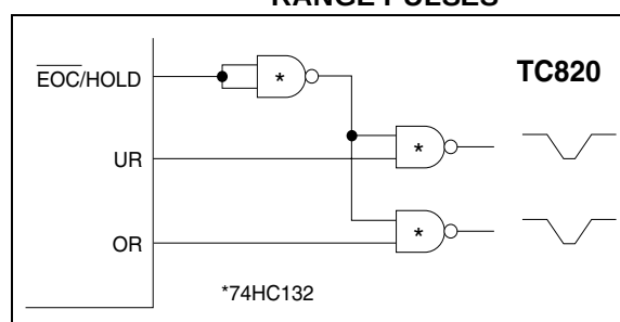
FIGURE 4-2: GENERATING UNDER RANGE AND OVER RANGE PULSES
