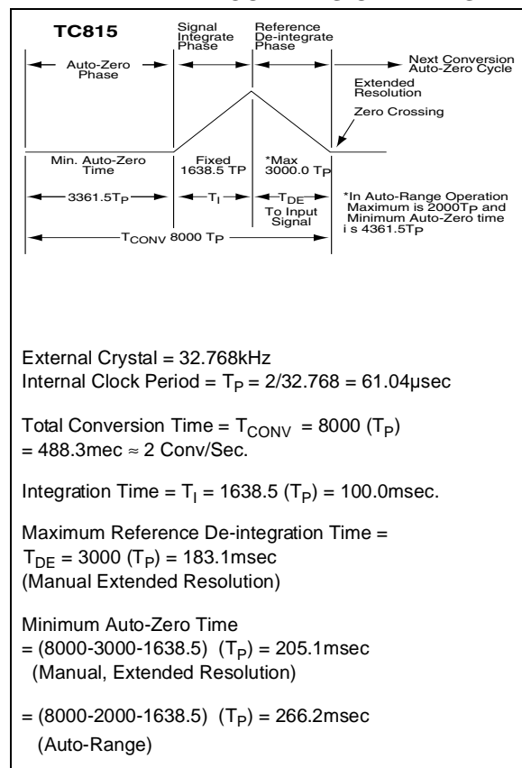
FIGURE 4-1: BASIC TC815 CONVERSION TIMING
