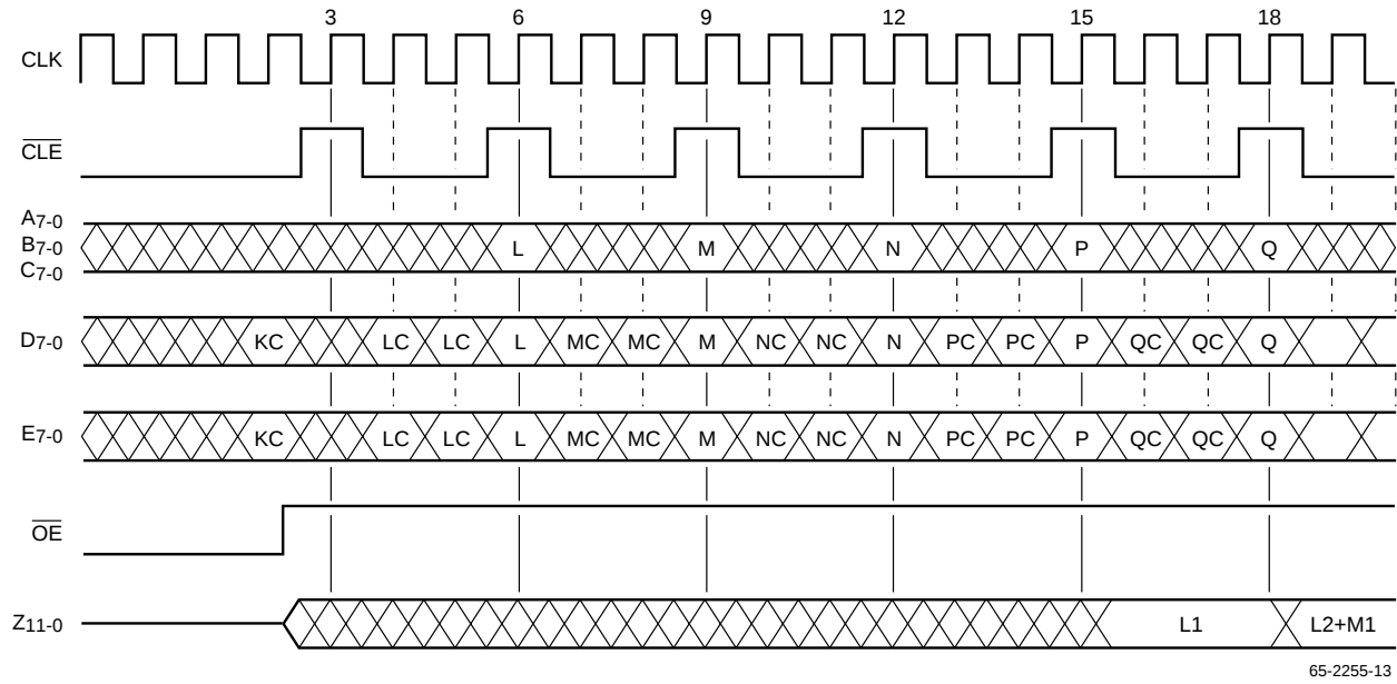
Figure 10. 5x5 Convolution, Periodic Short \overline{CLE} Pulse
