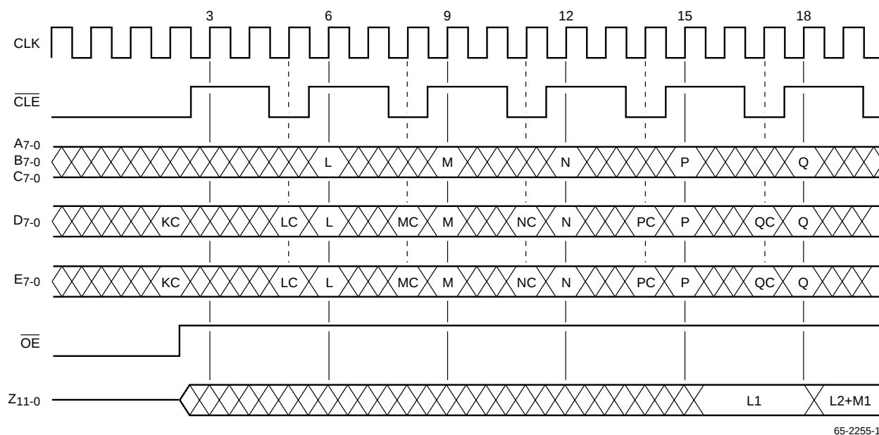
Figure 9. 5x5 Convolution, Periodic Long \overline{CLE} Pulse
