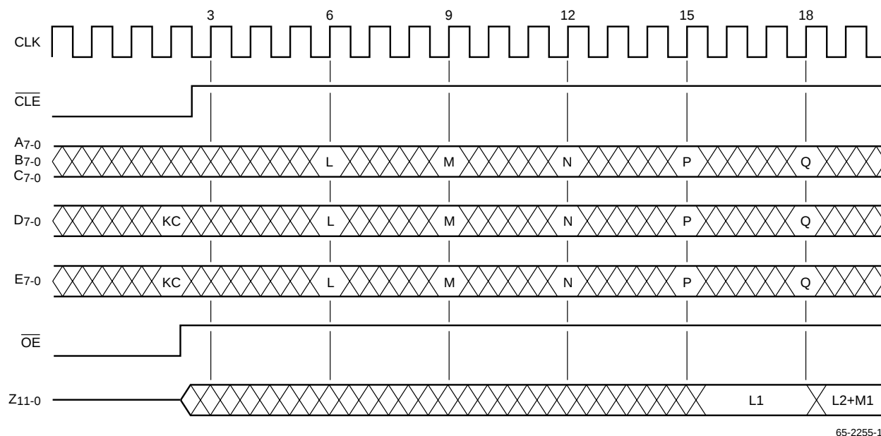
Figure 8. 5x5 Convolution, Single \overline{CLE} Rising Edge
