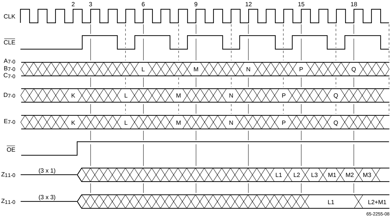
Figure 5. 3xX Modes, Periodic Long \overline{\text{CLE}} Pulses
