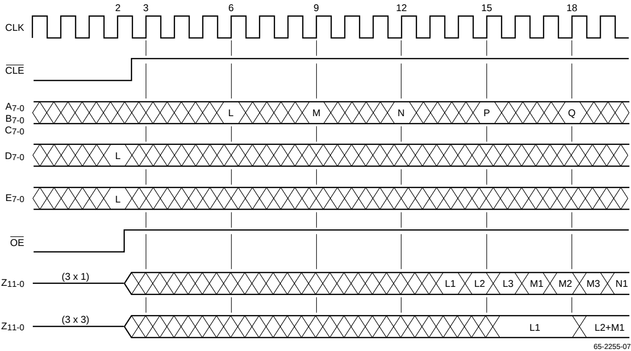
Figure 4. 3 (3x1), 3x3 Timing Diagram, Single \overline{\text{CLE}} Rising Edge
