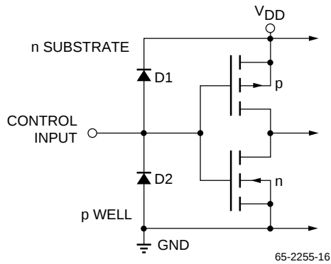
Figure 13. Equivalent Input Circuit
