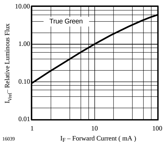
Figure 11. Relative Luminous Intensity vs. Forward Current
