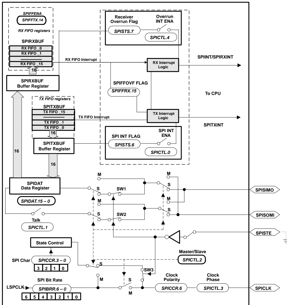
Figure 24. Serial Peripheral Interface Module Block Diagram
