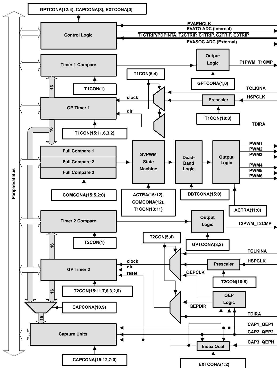
Figure 17. Event Manager A Functional Block Diagram
