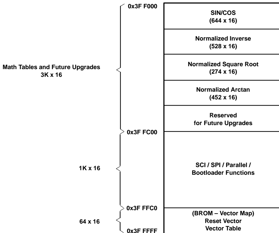
Figure 12. On-Chip Boot ROM Map
