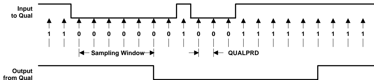
Figure 26. I/P Qualifier Clock Cycles
