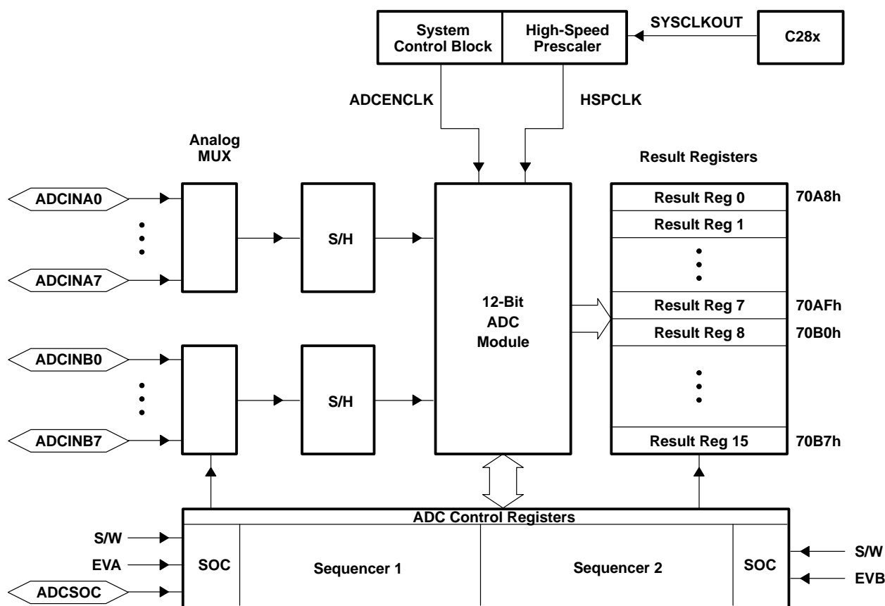
Figure 18. Block Diagram of the F2810 and F2812 ADC Module
