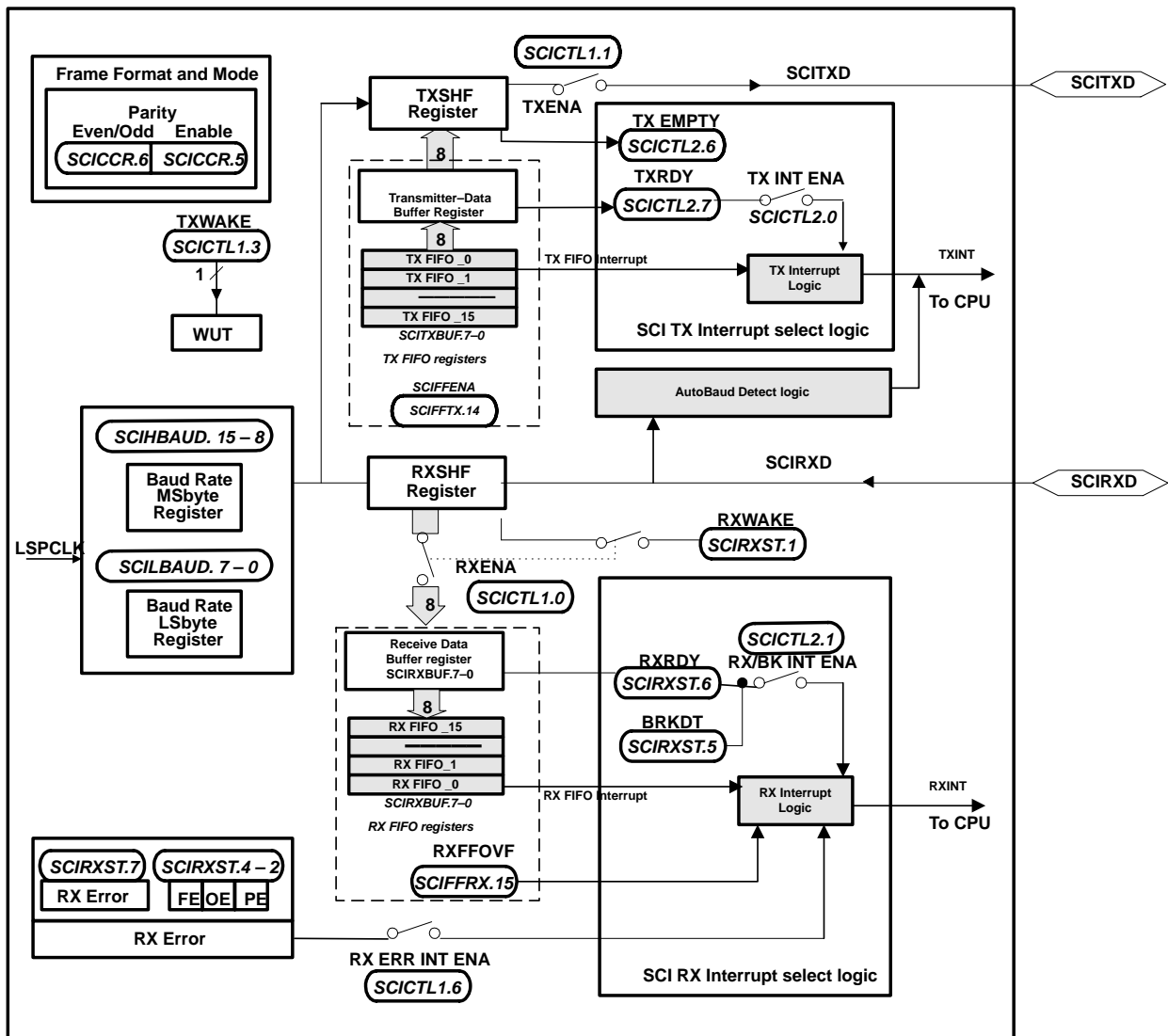
Figure 23. Serial Communications Interface (SCI) Module Block Diagram
