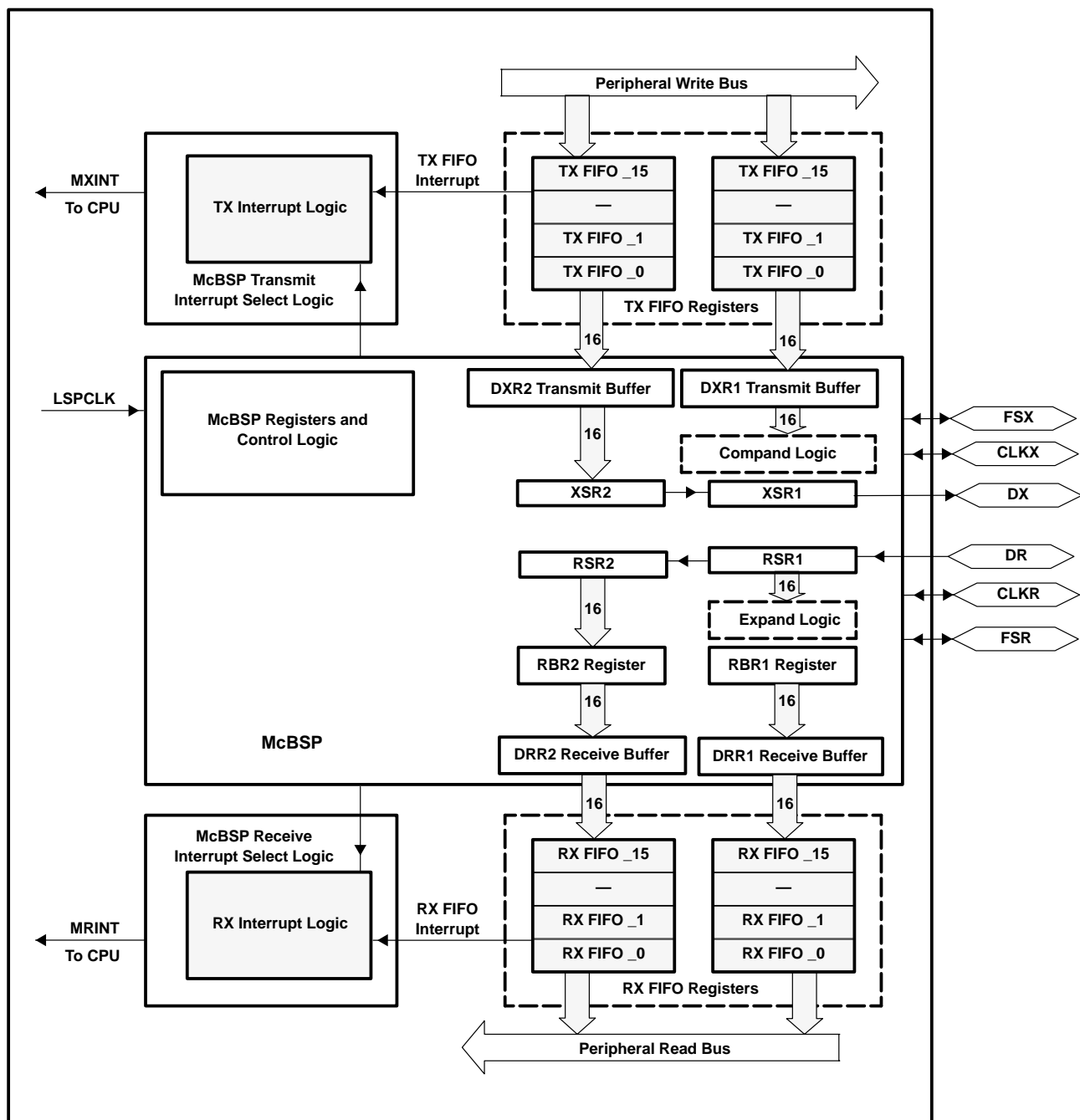
Figure 22. McBSP Module With FIFO
