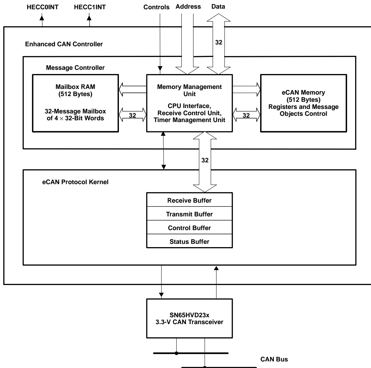
Figure 20. eCAN Block Diagram and Interface Circuit
