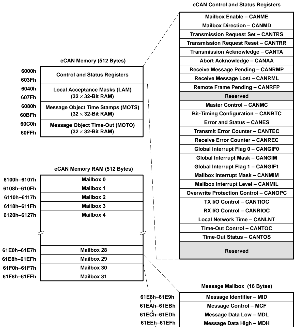
Figure 21. eCAN Memory Map
