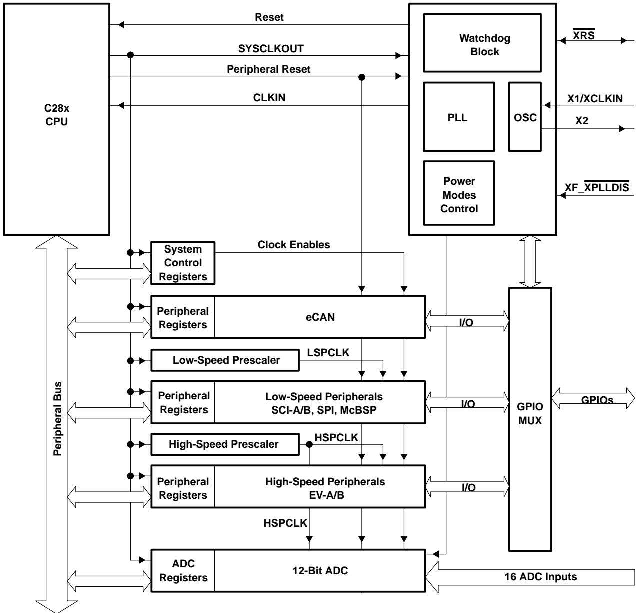
Figure 9. Clock and Reset Domains
