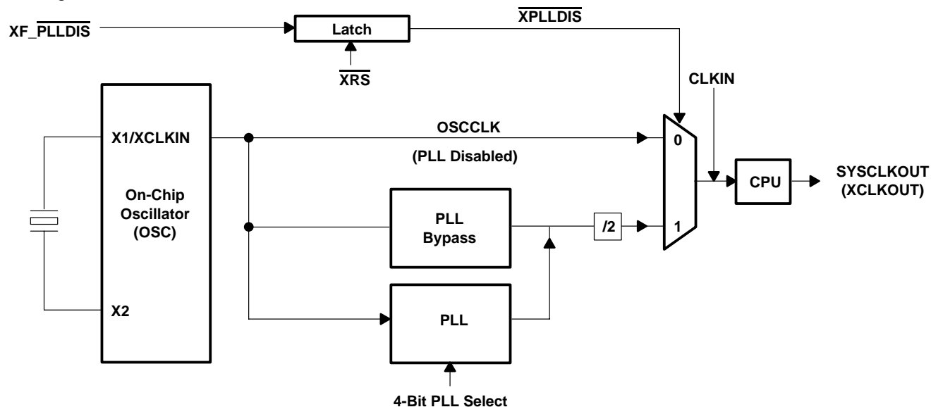
Figure 10. OSC and PLL Block
