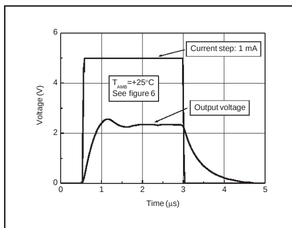
Pulse response for I_K = 1 \text{ mA}
