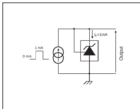
Figure 6 : Test Circuit for Response time
