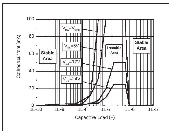
Stability behaviour with capacitive loads
