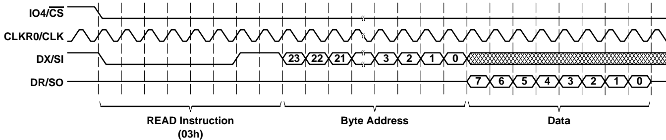
Figure 5. SPI EEPROM Mode Transfer Protocol With 24-Bit Addresses
