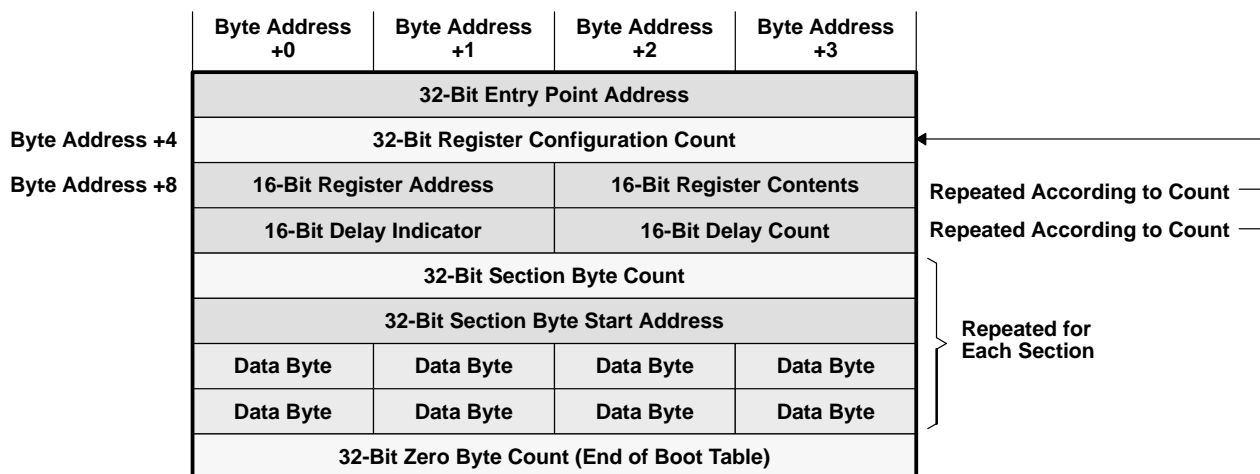
Figure 6. Boot Table Structure
