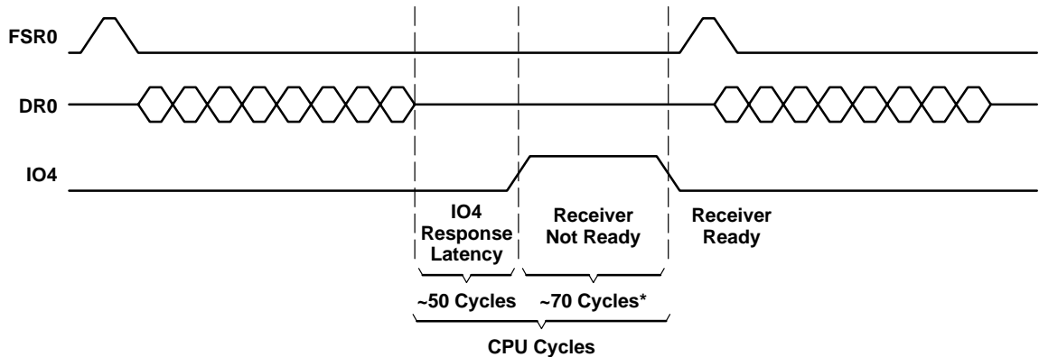
Figure 2. IO4 Latency for Boot-Table-Programmed Delays
