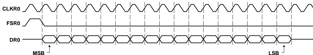
Figure 1. McBSP0 Receive Data Format for Bootload (16-Bit Shown)
