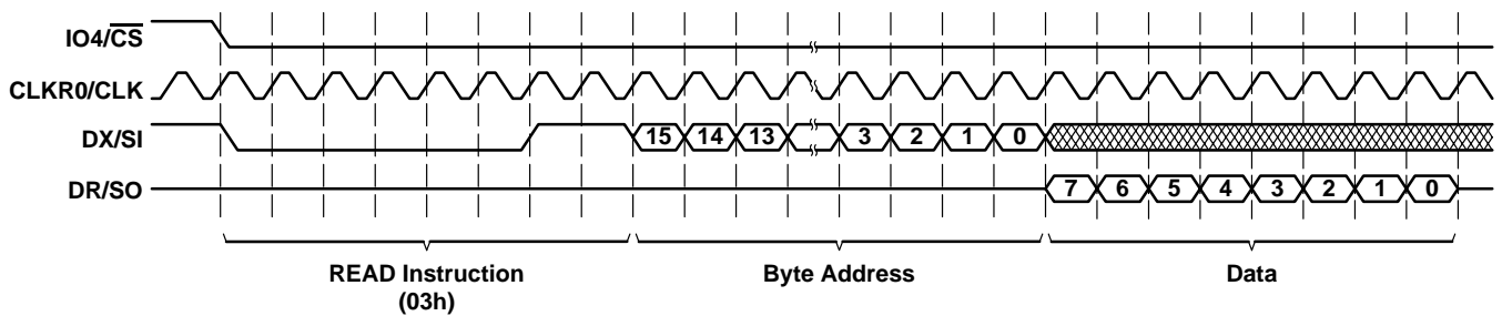
Figure 4. SPI EEPROM Mode Transfer Protocol With 16-Bit Addresses
