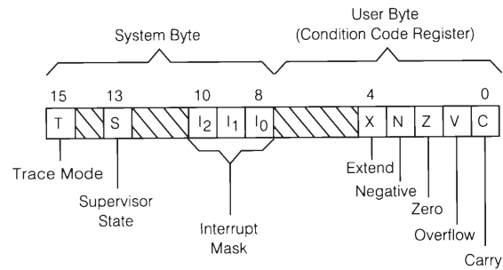
Figure 14 : Status register.
