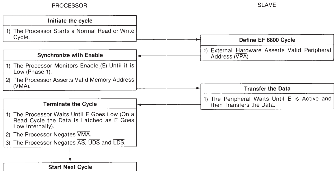
Figure 15 : EF 6800 interfacing flowchart.
