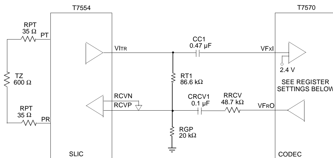
Figure 7. 600 \Omega Resistive SLIC Interface
