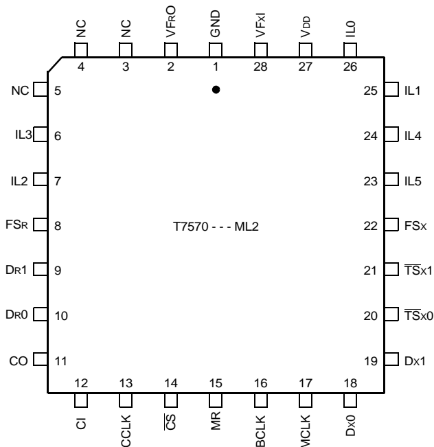
Figure 2. Pin Diagram
