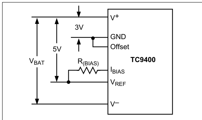
FIGURE 2: TC9400 supply and reference voltages.
