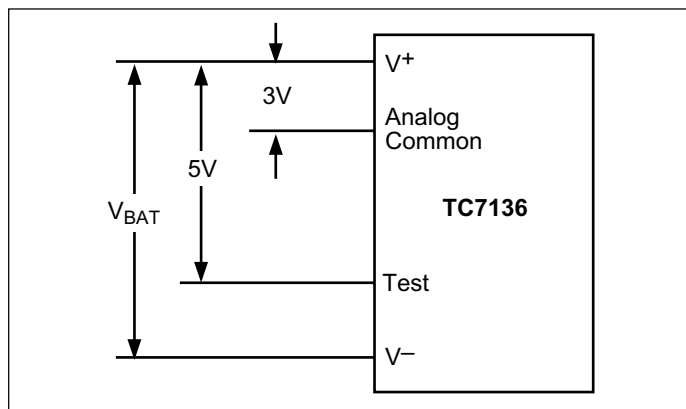
FIGURE 1: TC7136 regulated outputs.
