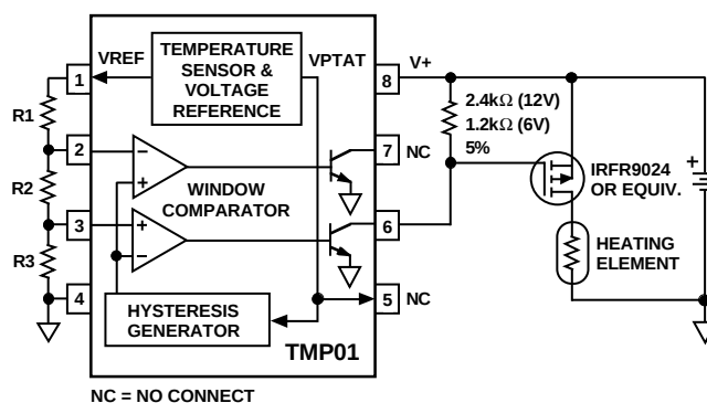
Figure 15b. Driving a P-Channel MOSFET
