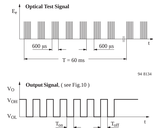
Figure 8. Output Function
