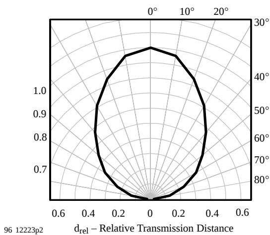
Figure 12. Directivity
