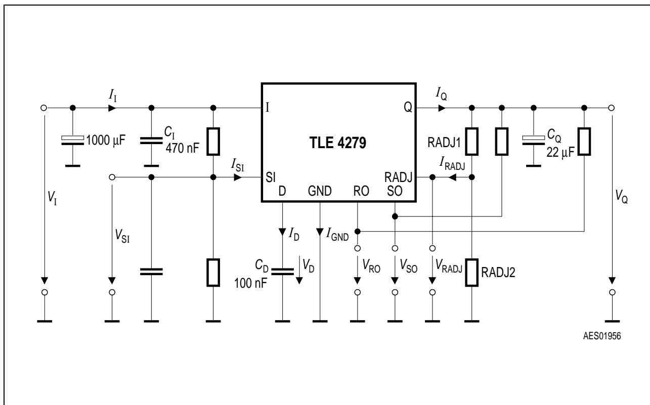
Figure 4 Measuring Circuit
