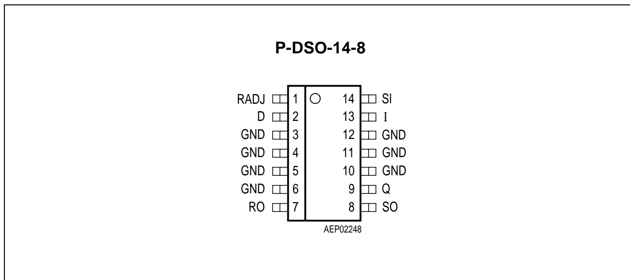
Figure 2 Pin Configuration (top view) (cont'd)
