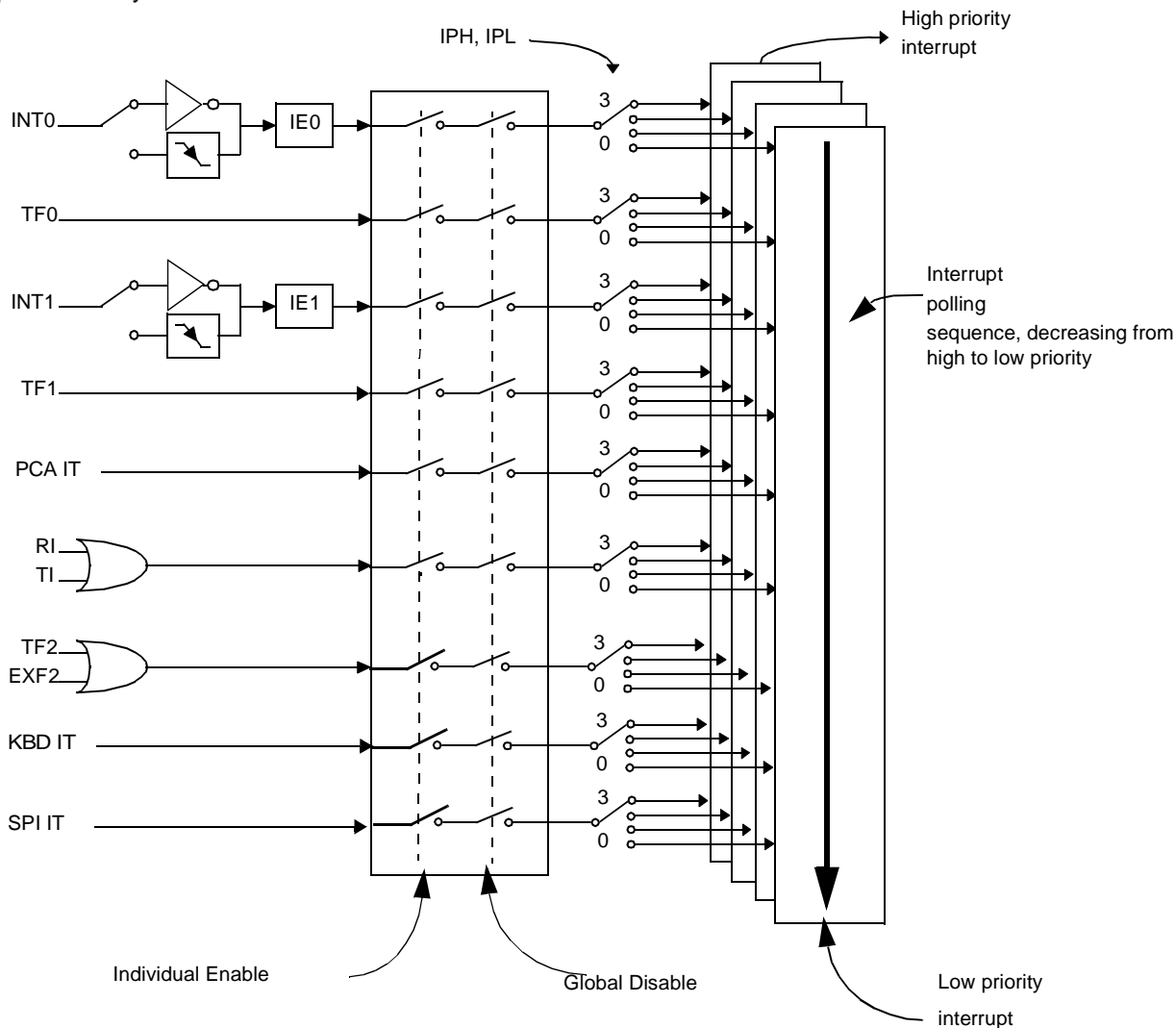
Figure 21. Interrupt Control System
