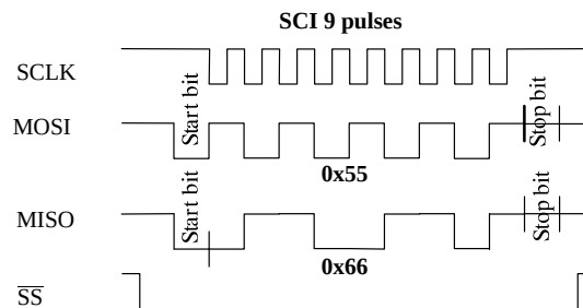
Figure 9. SCI data stream
