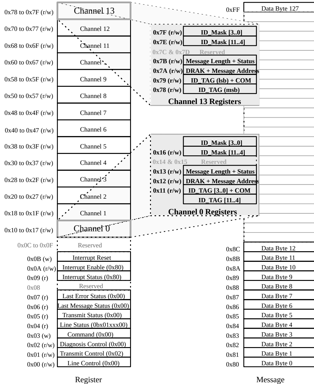
Figure 16. Memory Map.
