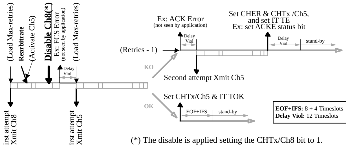
Figure 35. Disable channel after rearbitrate example
