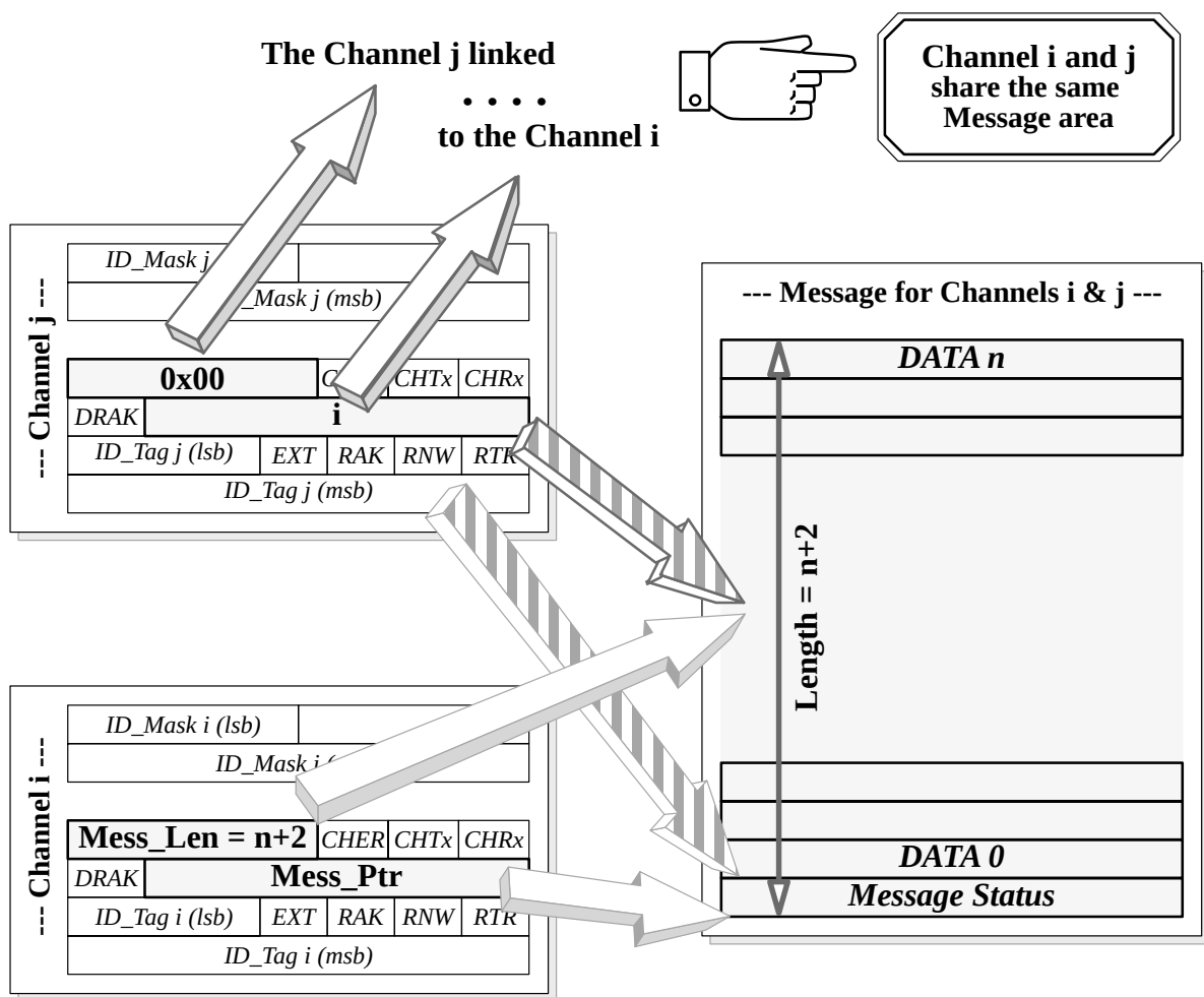
Figure 38. Linkage mechanism
