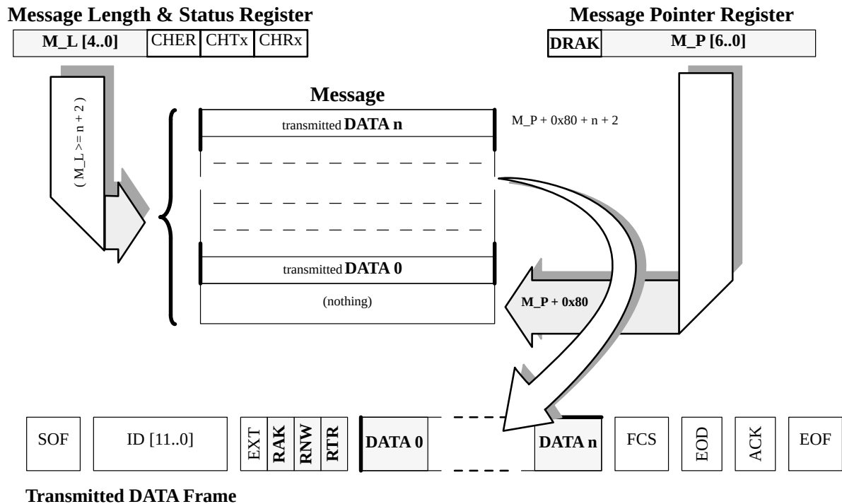
Figure 30. Message buffer structure for transmission
