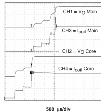
STARTUP TIMING
