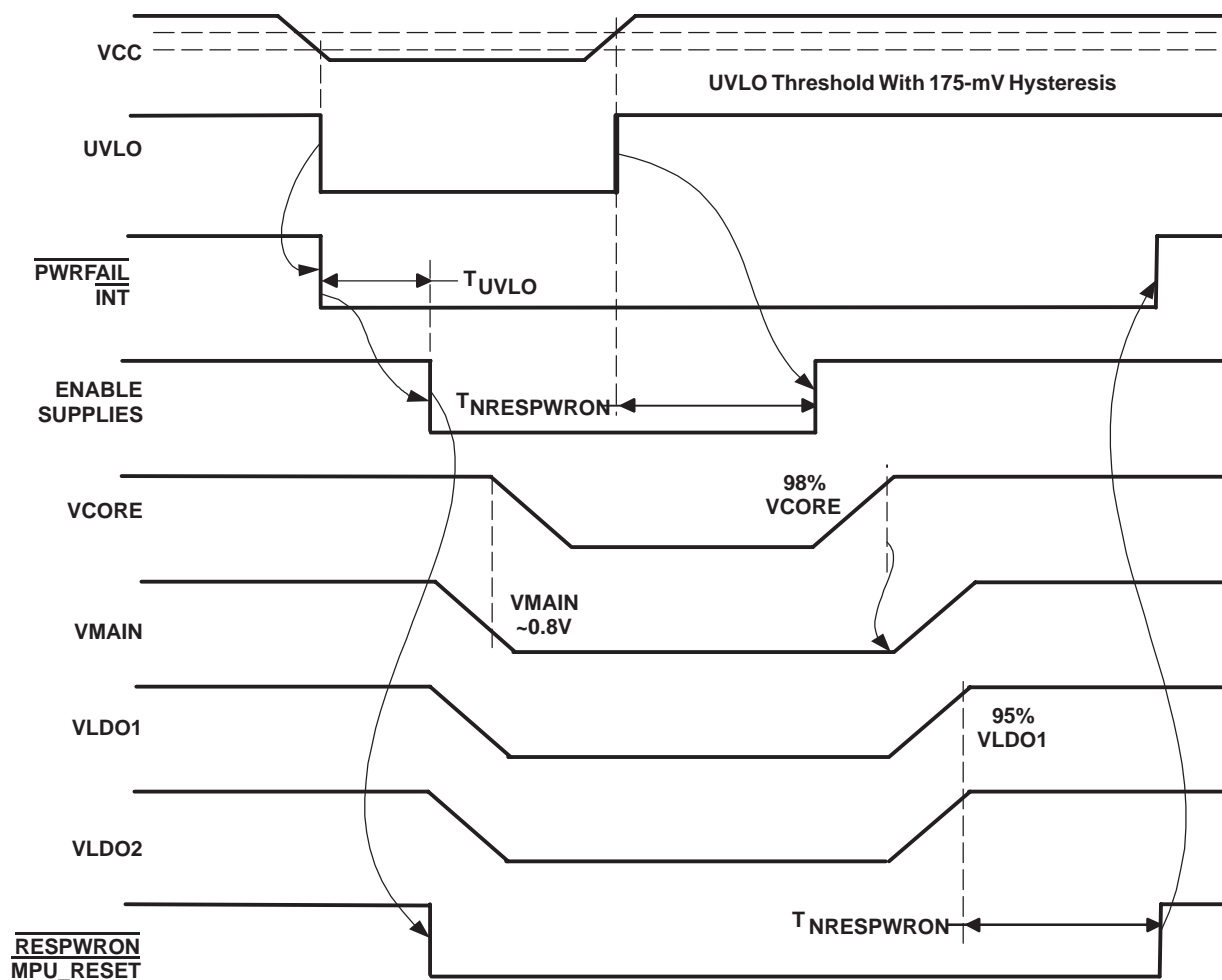
Figure 34. State2-State4-State 2 Transition
