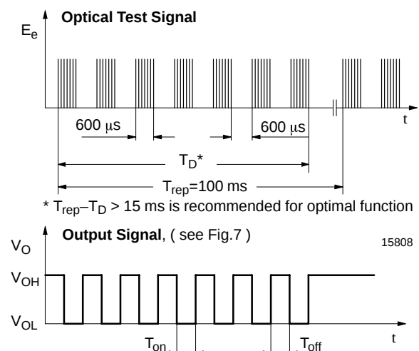
Figure 6. Output Function
