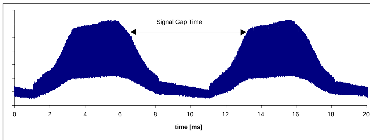
Figure B: Disturbance Signal from Fluorescent Lamp with Signal Gap Time of 7ms (suppressed by TSOP28..)
