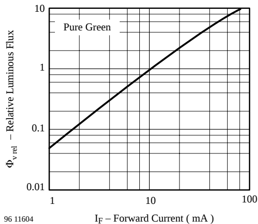
Figure 28. Relative Luminous Flux vs. Forward Current
