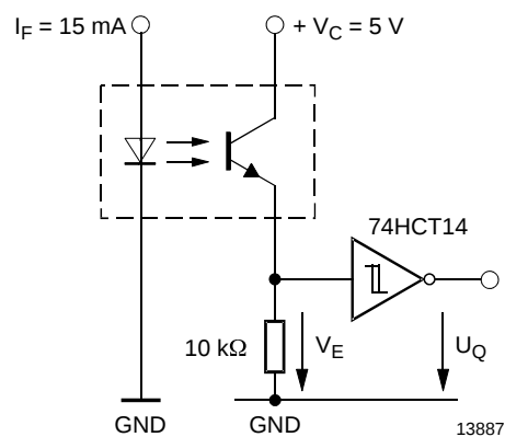
Figure 2. Application example
