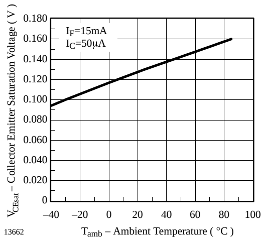
Figure 4. Collector Emitter Saturation Voltage vs. Ambient Temperature
