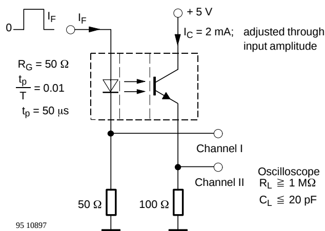
Figure 1. Test circuit, saturated operation
