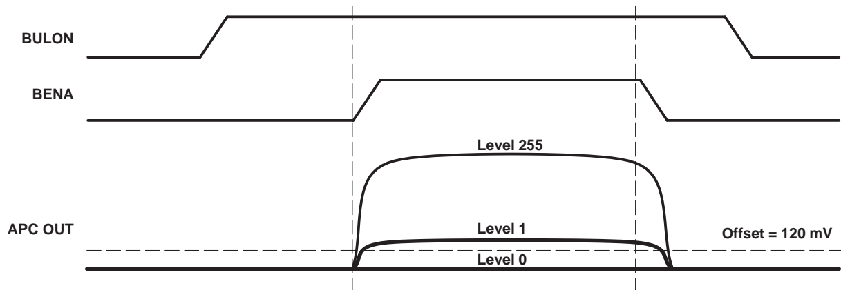
Figure 12. APC Output When APCMODE = 0
