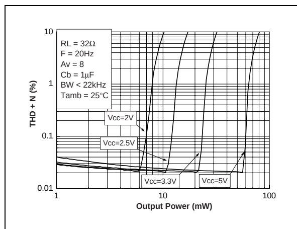
Fig. 81: THD + N vs Output Power
