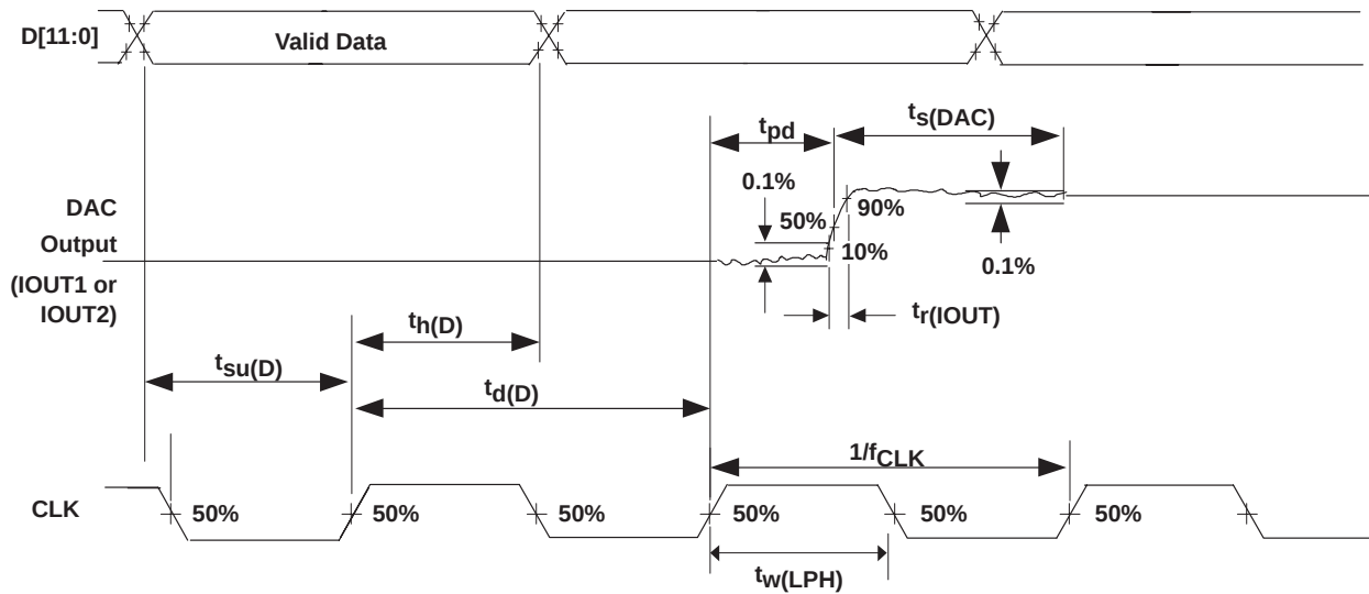
Figure 23. Timing Diagram
