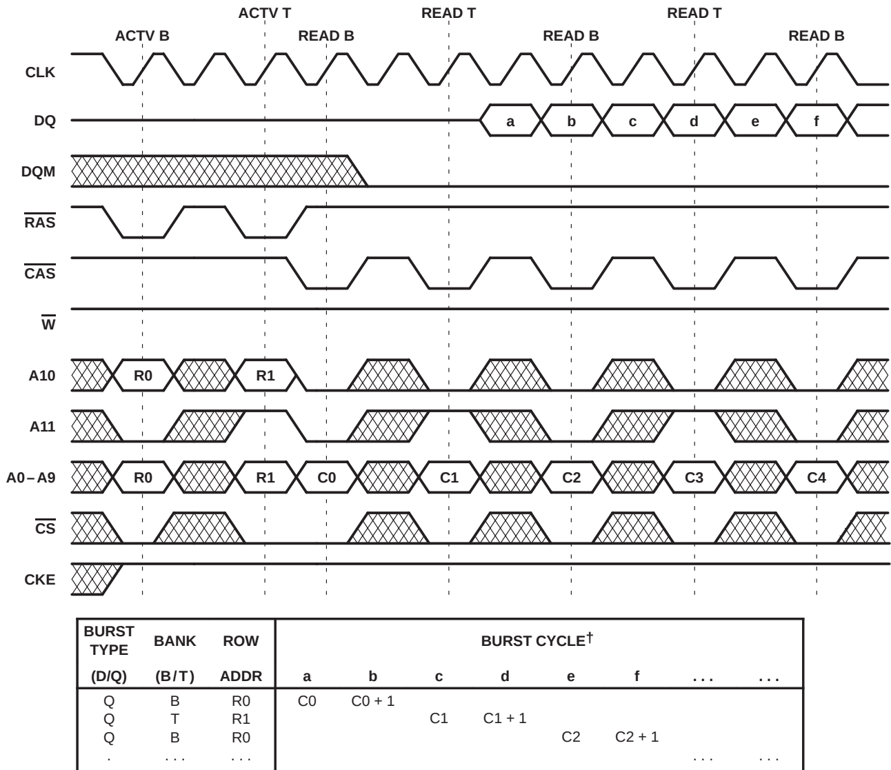
Figure 25. Two-Bank Column-Interleaving Read Bursts (CAS latency = 3, burst length = 2)
