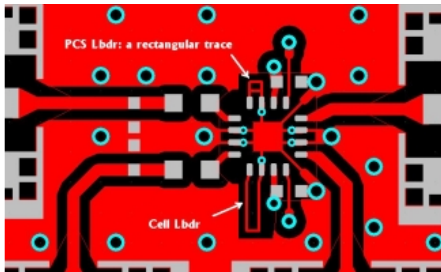
Figure 2 Showing Lbrd and Grounding on Evaluation Board
