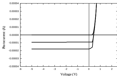
Fig. 2 Typical Photo-Current
