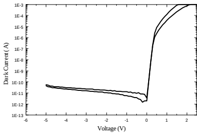
Fig. 1 Typical Dark Current and Forward Current
