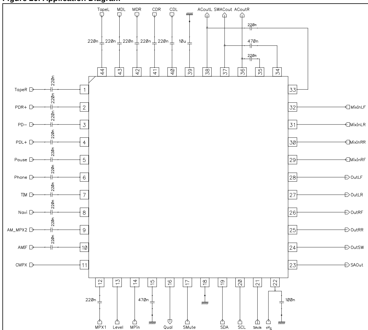
Figure 29. Application Diagram
