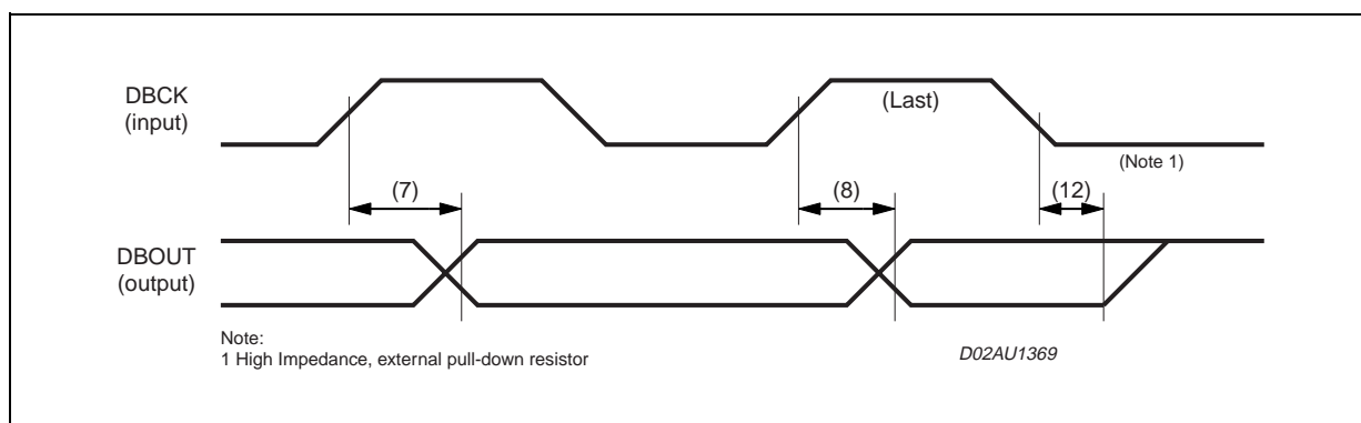
Figure 10. Debug Port Read Timing.
