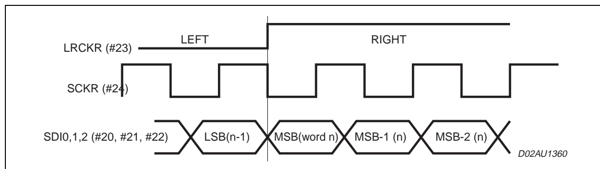
Figure 5. SAI protocol when RLRS=0; RREL=1; RCKP=1; RDIR=0.
