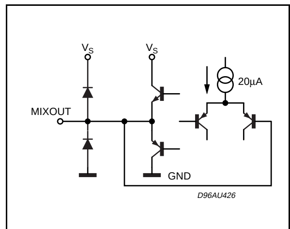
PINS: 8, 10
