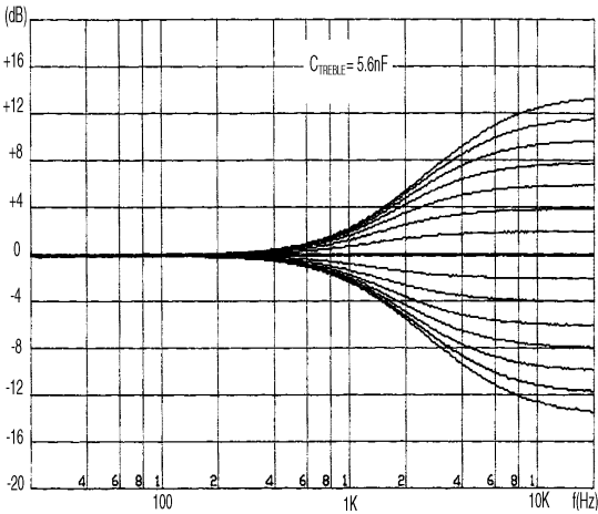
Figure 6: Treble response
