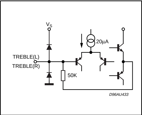
PINS: 18, 19
