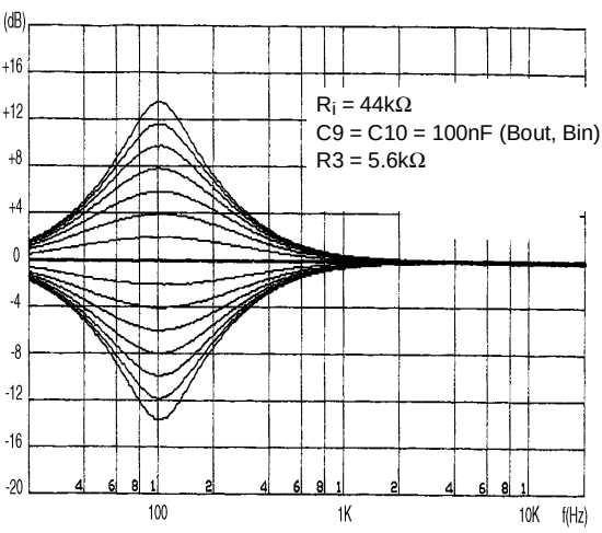
Figure 5: Bass response
