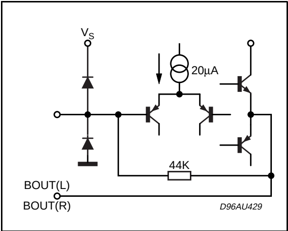
PINS: 13, 15
