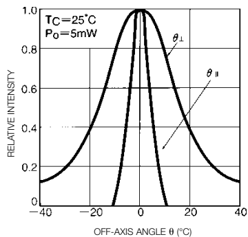
Far-field Patterns
