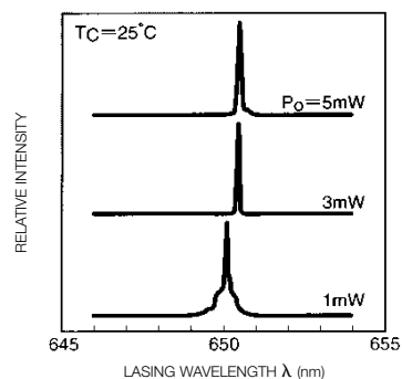
Lasing Spectrum
