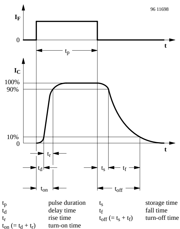
Figure 5. Switching times
