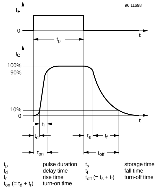
Figure 2. Switching times
