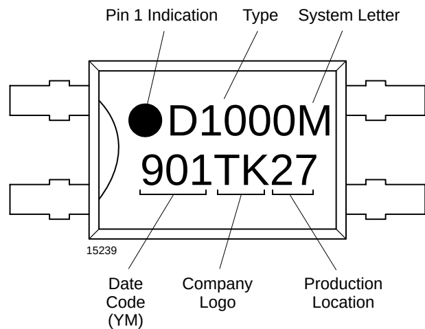
Figure 11. Marking example
